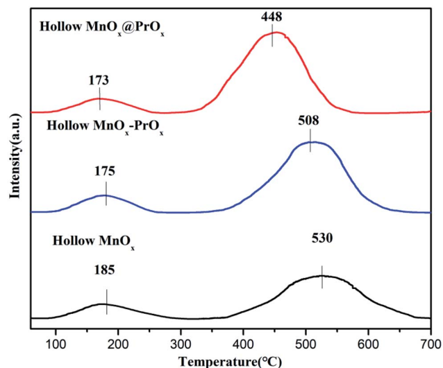
Fig. 8 NH 3 -TPD profiles of the catalysts.
