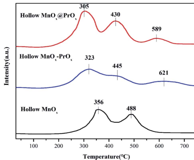
Fig. 9 H 2 -TPR profiles of the catalysts.
