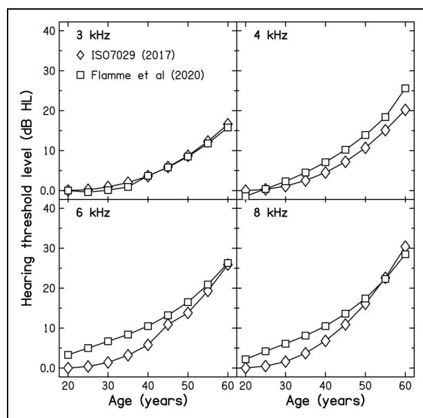
Figure 1. AAHL values for men expected from the 50 th percentile of ISO 7029 (2017) (diamonds) and from the values published by Flamme et al. (2020) (squares), plotted as a function of age. Each panel shows results for one frequency.
