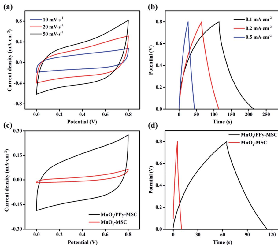
Fig. 4 (a) Cyclic voltammetry and (b) galvanostatic charge–discharge curves of \text{MnO}_2/\text{PPy-MSC} . (c) Comparison of CV and (d) GCD of \text{MnO}_2/\text{PPy-MSC} and \text{MnO}_2\text{-MSC} .
