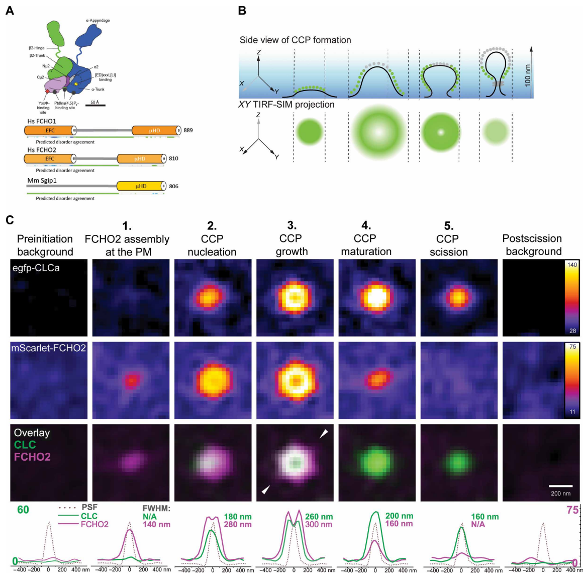
Fig. 1. Dual-color live-cell microscopy with high-NA eTIRF-SIM reveals dynamic nanoscopic FCHO2 assembly that predetermines site and size of CCP formation. (A) Cartoon representations of mammalian AP2 and muniscin family members FCHO1, FCHO2, and SGIP. AP2 is colored according to subunits as used throughout \alpha (dark blue), \beta 2 (dark green), \mu 2 (dark purple), \mu 1 (pale purple), and \sigma 2 (cyan). Muniscins have FBAR and MHD domains joined by unstructured interdomain linkers. (B) Top: Side-view representation of a forming CCP imaged by eTIRF-SIM with an illumination depth of 100 nm (blue gradient). Clathrin is depicted either in green when visible or gray when not visible because of the exponentially decaying evanescent wave of TIRF. Bottom: 2D projection of clathrin (green) in a forming CCP along its axis of invagination into the plane of the PM. (C) eTIRF-SIM images of mScarlet-FCHO2 WT and egfp-CLCa in different phases of CCP formation. Region of interest (ROI) containing single CCPs in a time series was dissected into phases depending on the appearance of FCHO2 or egfp-CLCa. ROIs with individual CCPs in different phases were assembled into a z-stack and averaged across 150 CCPs in three different cells. The bottom row shows comparison of not normalized intensity distribution profiles (along the line indicated with white triangles) for CLC and FCHO2 (green and magenta, respectively) at different time points together with their full width at half maximum (FWHM). The black dotted line shows the measured point spread function (PSF). N/A, not applicable.
