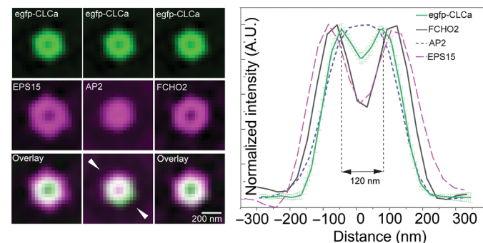
Fig. 2. FCHO, Eps15, AP2, and clathrin localization in CCPs. (Left) Averaged eTIRF-SIM images of multiple individual ROIs (as in C). The top row (green) shows CLC, and the middle row (magenta) shows pioneer proteins of interest (Eps15, AP2, and FCHO2). The bottom row demonstrates overlay between the channels highlighting the molecule distribution with respect to CLC. mScarlet-FCHO2 WT forms an annulus covering the outer rim of the clathrin hemispherical coat of averaged CLC (green line) that is 260 nm. (Right) Normalized egfp-CLCa intensity profiles along the line indicated with white triangles of the previous panel. The green solid line shows the CCP intensity profiles obtained from averaging images of 480 CCPs in U-2 OS cells with an estimated FWHM of 260 nm. While AP2 ( \alpha -adaptin egfp, shown in blue dashed line) forms a central patch in a mature CCP, Eps15 (polyclonal antibody, magenta dashed line) forms a transition zone with FWHM larger than that of FCHO2 (black) and egfp-CLCa (green). A.U., arbitrary units.
