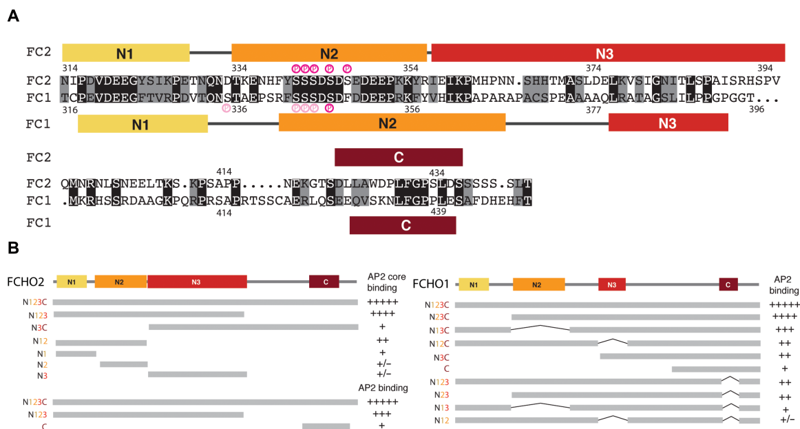
Fig. 4. Four sequence blocks in FCHO linkers and the effects of their deletion on AP2 binding. (A) Human FCHO2 (FC2 top) and FCHO1 (FC1 bottom) interdomain linker sequences aligned with identities highlighted in black and conservation in gray. Consensus CK2 phosphorylation sites are shown in dark pink and hierarchical CK2 sites in light pink. The conserved sequence blocks N1, N2, N3, and C assessed on the basis of conservations between sequences from across species and in the case of FCHO2, also on the basis of structure, are colored yellow, orange, red, and claret, respectively (coloring maintained throughout all subsequent figures). (B) Summary of the binding of the deletion constructs indicated on the unstructured FCHO2 and FCHO1 linkers to recombinant AP2 core and AP2 from brain cytosol as indicated. Gels shown in fig. S3.
