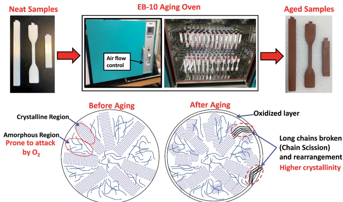
Fig. 6 Physical and intrinsic structure changes of a semicrystalline polymer in high temperature aging oven.
