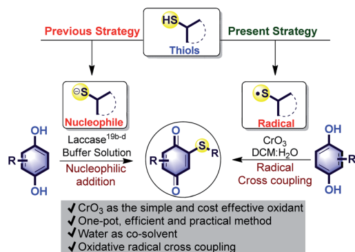
Scheme 1 Quinonyl thioethers from thiol and hydroquinone.
