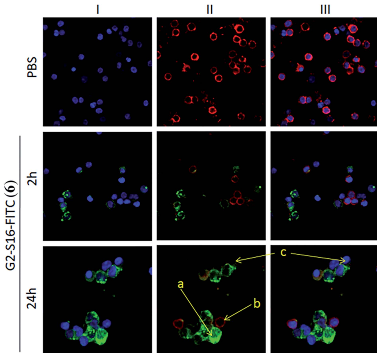
Fig. 2 Confocal microscopy images of ability of the polyanionic CBS dendrimer G2-S16-FITC ( 6 ) to enter into PBMCs. (I) G2-S16-FITC dendrimer co-located with nuclei of treated cells labelled with DAPI; (II) anti-human CD4-APC co-located with G2-S16-FITC dendrimer; (III) represents co-localization of G2-S16-FITC dendrimer, CD4 and nuclei of treated cells labelled with DAPI. Arrows point different cell types (a) macrophage; (b) CD4 T lymphocyte; and (c) CD8 T lymphocyte.
