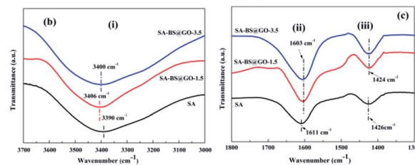
Fig. 4 FT-IR spectra of the SA and SA-BS@GO-X hybrid membranes: (a) whole spectra; (b) spectra of region (i); (c) spectra of regions (ii) and (iii).
