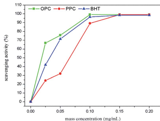
Fig. 11 ABTS •+ scavenging capacity of OPC, PPC and BHT at different mass concentrations.
