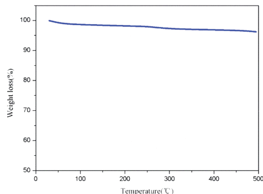
Fig. 5 TG chart for Pd/C-SO 3 H.
