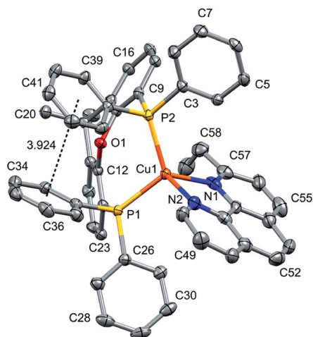
Fig. 4 Structure of the [Cu(xantphos)(2-Etphen)] + cation with ellipsoids plotted at 50% probability, H atoms are omitted for clarity. Negligible \pi -interaction between two of the phenyl rings on the different phosphorus atoms (involving C34 and C39, respectively) (angle between the ring planes 27.10°, centroid-centroid distance 3.924 Å), but none involving the xanthene backbone.
