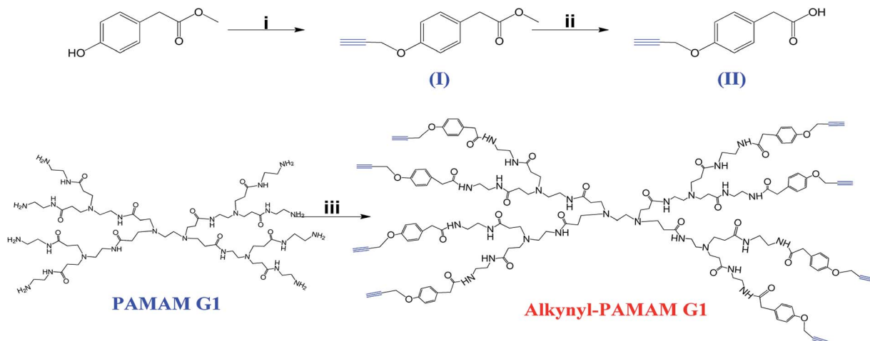
Scheme 1 Synthesis of alkynyl-PAMAM G1. Conditions: (i) propargyl bromide, K_2CO_3 , anhydrous acetone, 24 h, reflux; (ii) NaOH/HCl, EtOH : H_2O ; (iii) EDC, HOBt, DIPEA, DMF, 35^\circ C , 5 days.
