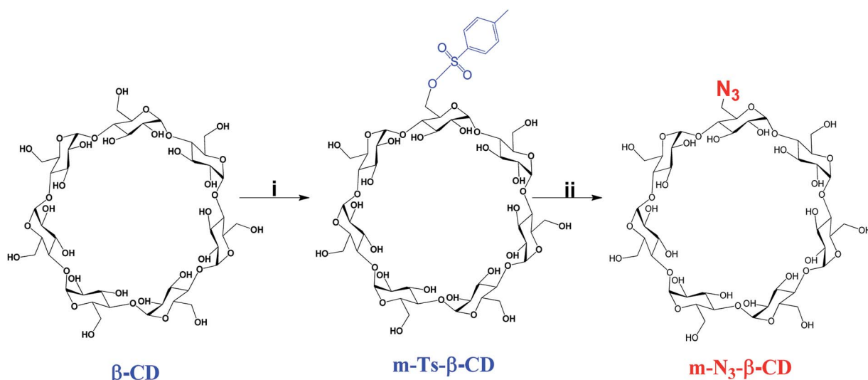
Scheme 2 Synthesis of m-N_3 - \beta -CD. Conditions: (i) TsO_2/NaOH , H_2O , 2 h, RT; (ii) NaN_3 , DMF, 80^\circ C , 48 h.
