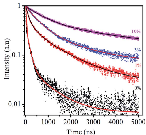
Fig. 8 PL-decay kinetics of \text{Zn}_{0.5}\text{Cd}_{0.5}\text{Se}:\text{Cu} ( y\% , y = 0, 1, 3, 10 ) alloy QDs excited at 488\text{ nm} , measured at the emission peak of Cu and/or the surface. The solid lines are fitting curves to a multi-exponential function.
