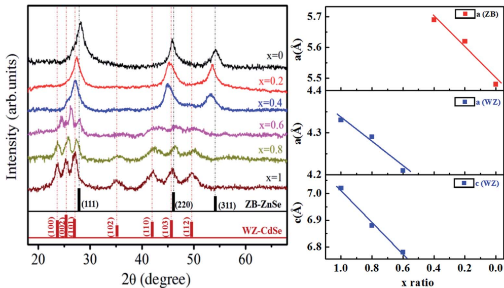
Fig. 3 (Left) XRD pattern and (Right) plot of lattice parameters 'a' and 'c' versus composition of Zn 1-x Cd x Se (0 ≤ x ≤ 1):Cu 0.5% alloy QDs for hexagonal and cubic structure.
