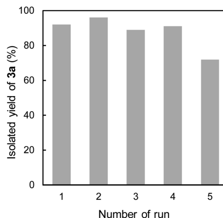
Fig. 2 Recyclability of CsNFs in Knoevenagel condensation.
