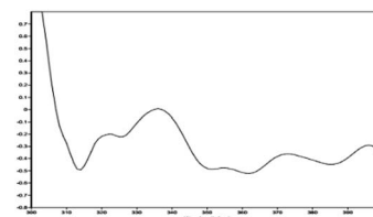
Fig. 4 The CD difference spectrum of Rh_2(OCOCF_3)_4 bind with compound 1.
