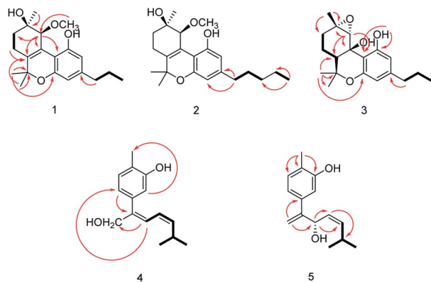
Fig. 2 Key 1 H- 1 H COSY —, HMBC → correlations of compounds 1-5.
