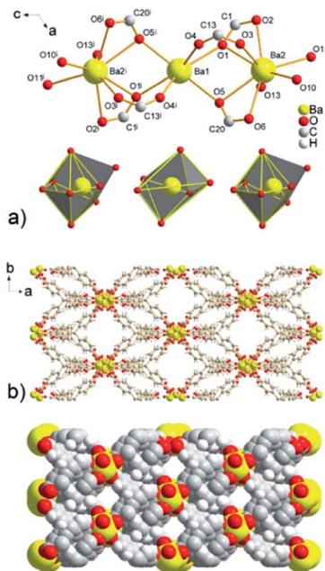
Fig. 5 (a) A view of the linear three-nuclear barium cluster with composition [\text{Ba}_3(\mu_2\text{-COO})_6(\text{H}_2\text{O})_6] in UPJS-9 (hydrogen atoms were omitted for clarity, i = -x, y, 1/2 - z ). (b) View of a 3D polymeric framework with 1D channels propagating along c crystallographic axis.
