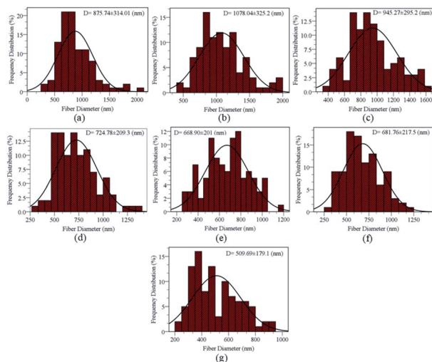
Fig. 6 (a–g) Fiber diameter distributions of electrospun nanofibers of PVDF/BaTiO 3 solution with PVDF concentration of 25 wt% and various BaTiO 3 concentrations of 6 wt%, 12 wt%, 18 wt%, 20 wt%, 22 wt%, 24 wt% and 26 wt%, respectively.
