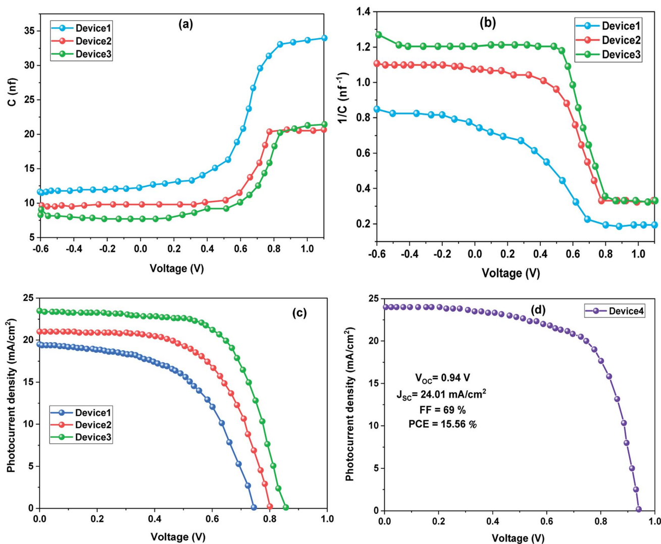
Fig. 4 (a) C - V measurements of HTM-free PSCs based on Au electrodes, (b) Mott-Schottky plot, (c) J - V curves of HTM-free PSCs based on Au electrodes, and (d) J - V curve of HTM-free PSC based on MWCNT electrode.
