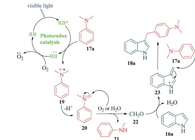
Scheme 6 Postulated mechanism for the Friedel–Crafts alkylation of indoles.
