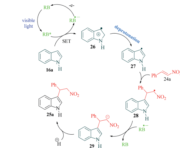
Scheme 8 Rose Bengal catalysed Friedel–Crafts alkylation of indoles.
