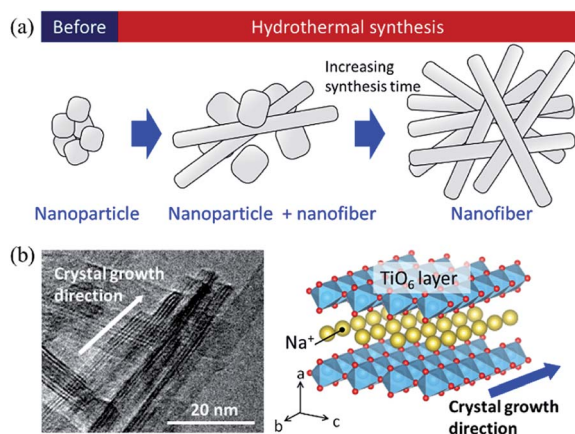
Fig. 6 (a) Schematic image of the formation of sodium dititanate nanofibre by hydrothermal synthesis, and (b) comparison of the growth direction between the TEM image and crystal structure model.
