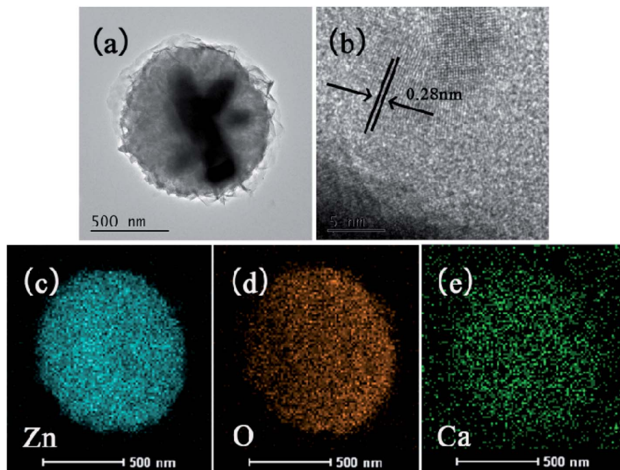
Fig. 2 TEM (a) and HRTEM (b) images of ZnO on the surface of ATC samples, and the corresponding elemental mapping results for Zn (c), O (d), Ca (e).
