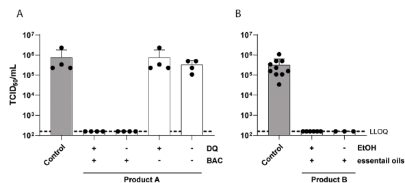
Fig. 1. Quantitative suspension test of commercially available mouthrinses. (A) Product A and (B) Product B of different compositions (white bars) or medium (grey bar) were incubated with SARS-CoV-2 and an interfering substance for 30 s. Viral titers were obtained by end point dilution on Vero E6 cells. Cytotoxicity is indicated as lower limit of quantification (LLOQ, dotted line). 50% tissue culture infectious dose (TCID 50 /mL) was calculated according to Spearman and Kärber. Data are represented as mean \pm SD of three independent experiments.
