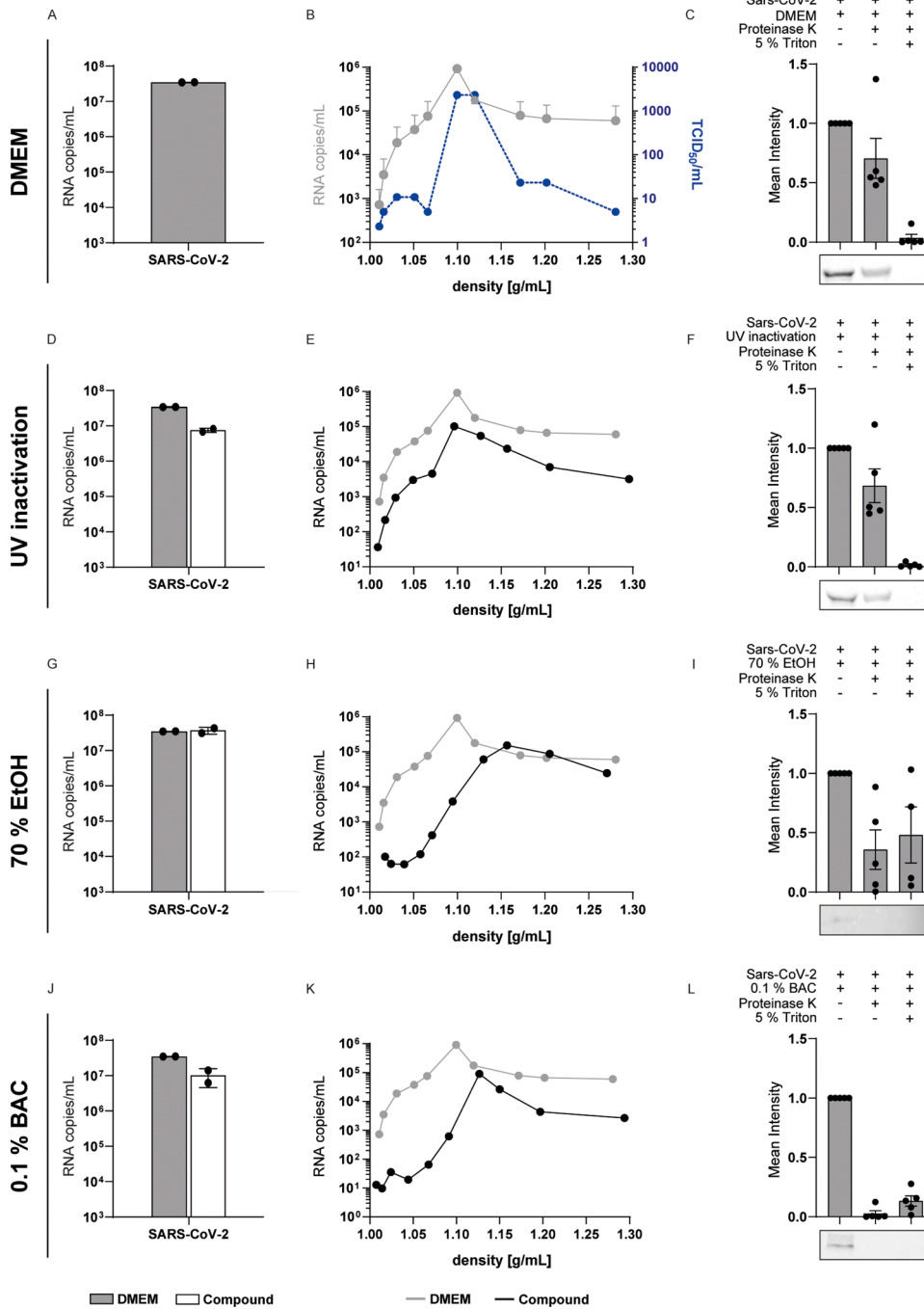
Fig. 3. Mode of action of antiseptic agents. SARS-CoV-2 was either incubated with DMEM (A-C), UV-inactivated (D-F), treated with 70% EtOH (G-I) or 0.1% BAC (J-L) and an interfering substance for 30 s. RNA integrity (A, D, G and J) for each treatment (white bar) was investigated by RT-qPCR and compared to DMEM (grey bar). Sucrose step gradient ultracentrifugation was performed to evaluate viral envelope integrity (B, E, H, K) and infectivity (blue line, B). RNA copy numbers in each fraction were determined by RT-qPCR (black line) and compared to DMEM (grey line). The viral envelope was further assessed by a capsid protection assay (C, F, I, L). Therefore, one replicate was left untreated, one part was treated with proteinase K for 1 h at 4 °C, and another part was lysed in 5% Triton X-100 prior to proteinase K treatment. The amount of protease-resistant nucleocapsid protein was quantified by Western blot. Data indicate averages.
