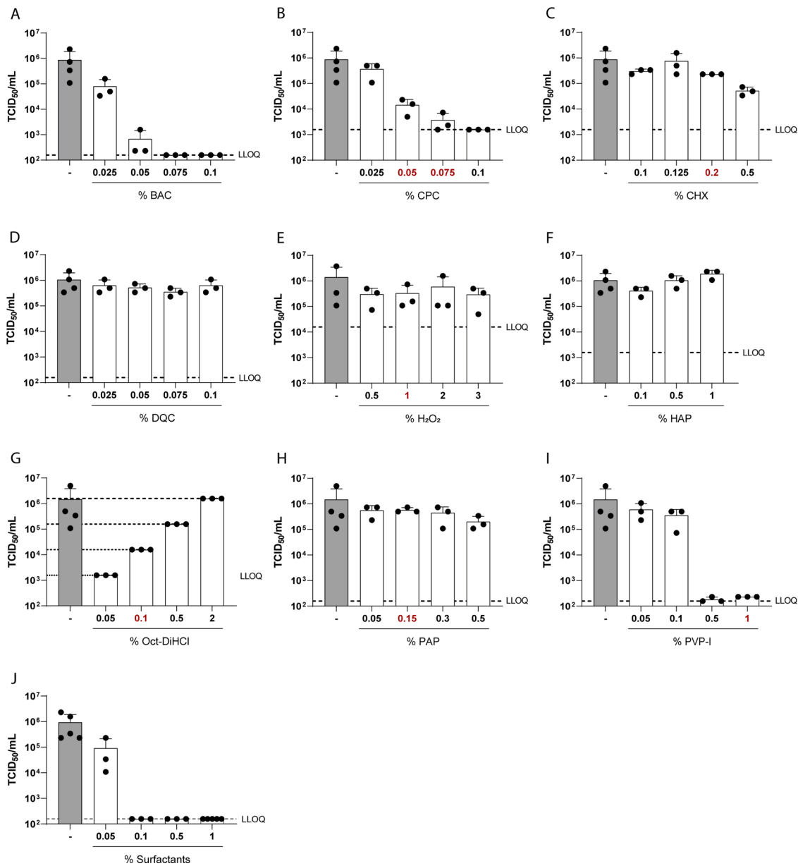
Fig. 2. Quantitative suspension test of antiseptic agents. (A-J) Antiseptic agents in various concentrations (white bars) or medium (grey bar) were incubated with SARS-CoV-2 and an interfering substance for 30 s. Viral titers were obtained by end point dilution on Vero E6 cells. Cytotoxicity is indicated as lower limit of quantification (LLOQ, dotted line). 50% tissue culture infectious dose (TCID 50 /mL) was calculated according to Spearman and Kärber. Red numbers indicate concentrations that appear in commercially available mouthrinses. Data are represented as mean ± SD of three independent experiments.
