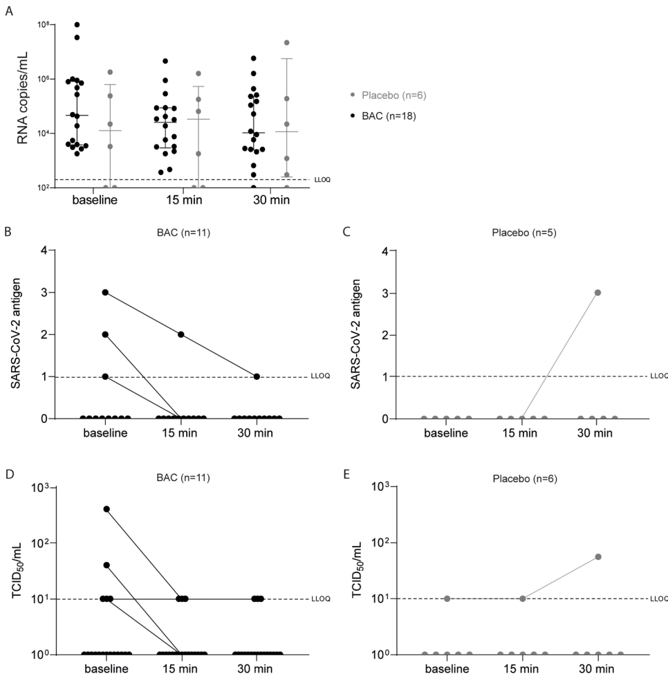
Fig. 4. In vivo activity of BAC against SARS-CoV-2. BAC was applied in a randomized placebo-controlled clinical trial in COVID-19 patients. RNA copy numbers were determined before gargling (baseline) as well as 15 and 30 min after gargling (A) comparing the placebo group (grey) to the BAC group (black). At similar time points SARS-CoV-2 antigen (B and C) and infectivity (D and E) was assessed for the BAC and placebo group, respectively. Data are shown as medians including 1st and 3rd quartiles.
