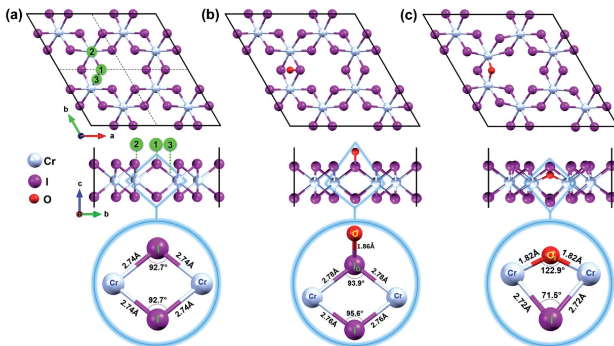
Fig. 1 Top and side views of (a) pristine \text{CrI}_3 monolayer. The black box displays the periodic supercell while dashed lines represent the boundaries of a unit cell. Oxygen was initially located 3 Å above at binding sites numbered as 1, 2, and 3 in green circles. Top and side view of (b) oxygen attached and (c) oxygen doped \text{CrI}_3 monolayer. The selected units of \text{CrI}_3 monolayer without and with oxygen defect are zoomed-in at the bottom panel of (a–c). The red, cyan, and purple balls belong to the O, Cr, and I-atoms, respectively.
