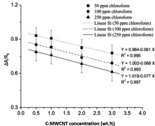
Fig. 18 Variation in sensor response toward CHCl 3 vapour as a function of c-MWCNT concentration in PANI/c-MWCNT nanocomposite. Reproduced from ref. 199, copyright 2015, Elsevier.
