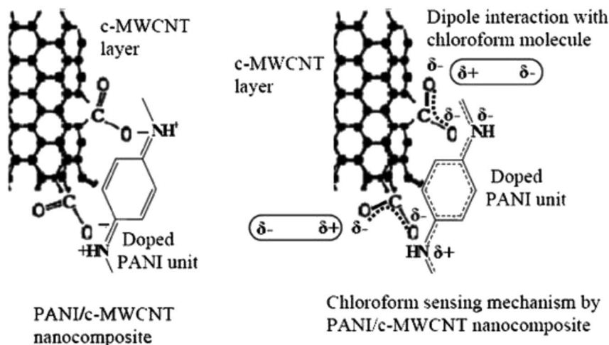
Fig. 17 Suggested mechanism of CHCl 3 molecules with PANI/c-MWCNT nanocomposite. Reproduced from ref. 199, copyright 2015, Elsevier.
