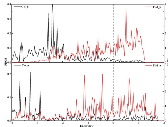
Fig. 8 The projected density of states plots of the sd^2 hybridization of the Ti atom corresponding to the local configuration in Fig. 5(a).
