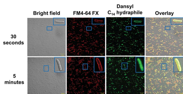
Fig. 3 Co-localization of FM4-64FX ( 5 \mu\text{g mL}^{-1} ) and dansyl C_{14} hydraphile in tet R E. coli . Top panel: FM4-64FX was fixed after 5 minutes and dansyl C_{14} hydraphile was fixed after 30 seconds. Bottom panel: FM4-64FX was fixed after 5 minutes and dansyl C_{14} hydraphile was fixed after 5 minutes. The scale bars are 10 \mu\text{m} (approximately the width of the smaller boxes).
