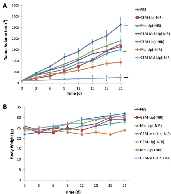
Fig. 9 In vivo antitumor effects of various treatments on BxPC-3 tumor-bearing mice. (A) Tumor growth curve following different treatments ( n = 5 ) (B) body weight as a function of days post-treatment for the indicated treatment groups. **P < 0.01 .
