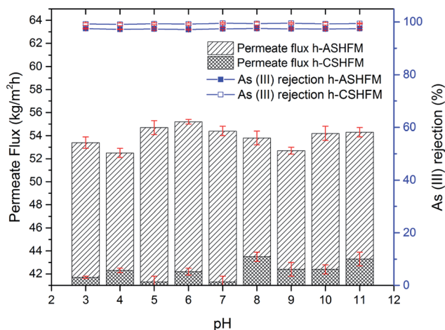
Fig. 4 Effect of pH on the permeate flux and As(III) rejection of h-ASHFM and h-CSHFMs sintered at 1200 ^\circ\text{C} , during the DCMD process (number of samples, n = 3 ; arsenic concentration = 1 ppm; arsenic feed temperature = 60 ^\circ\text{C} ).
