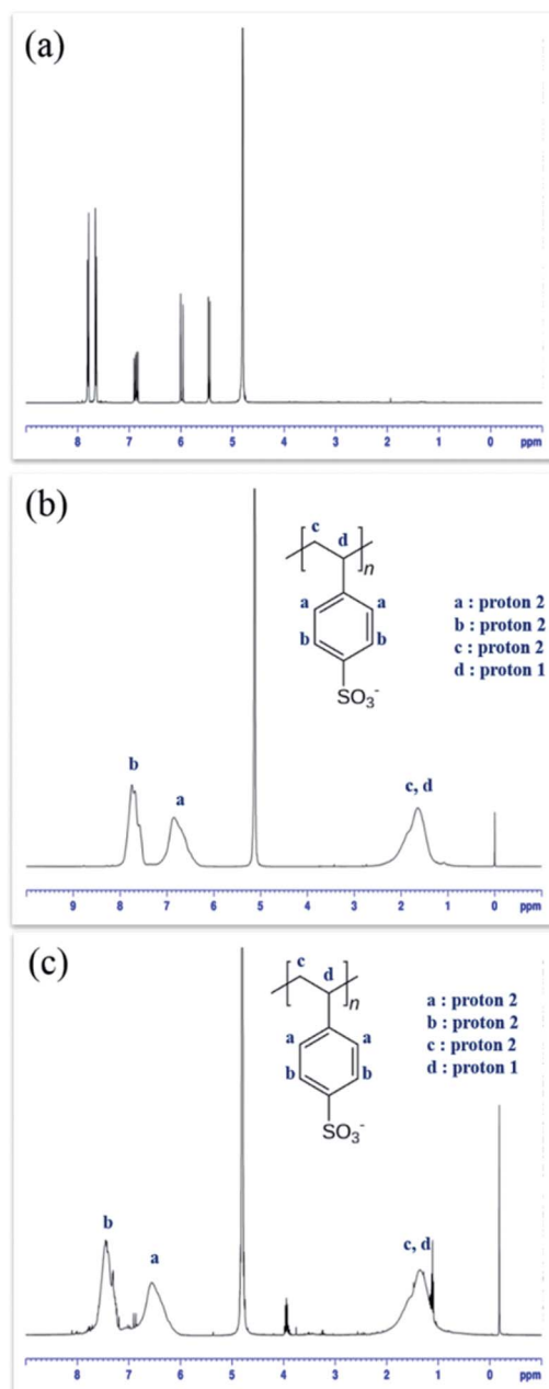
Fig. 3 1 H NMR spectra of NaSS (a), free radical PSSA (b), ATRP PSSA (c).
