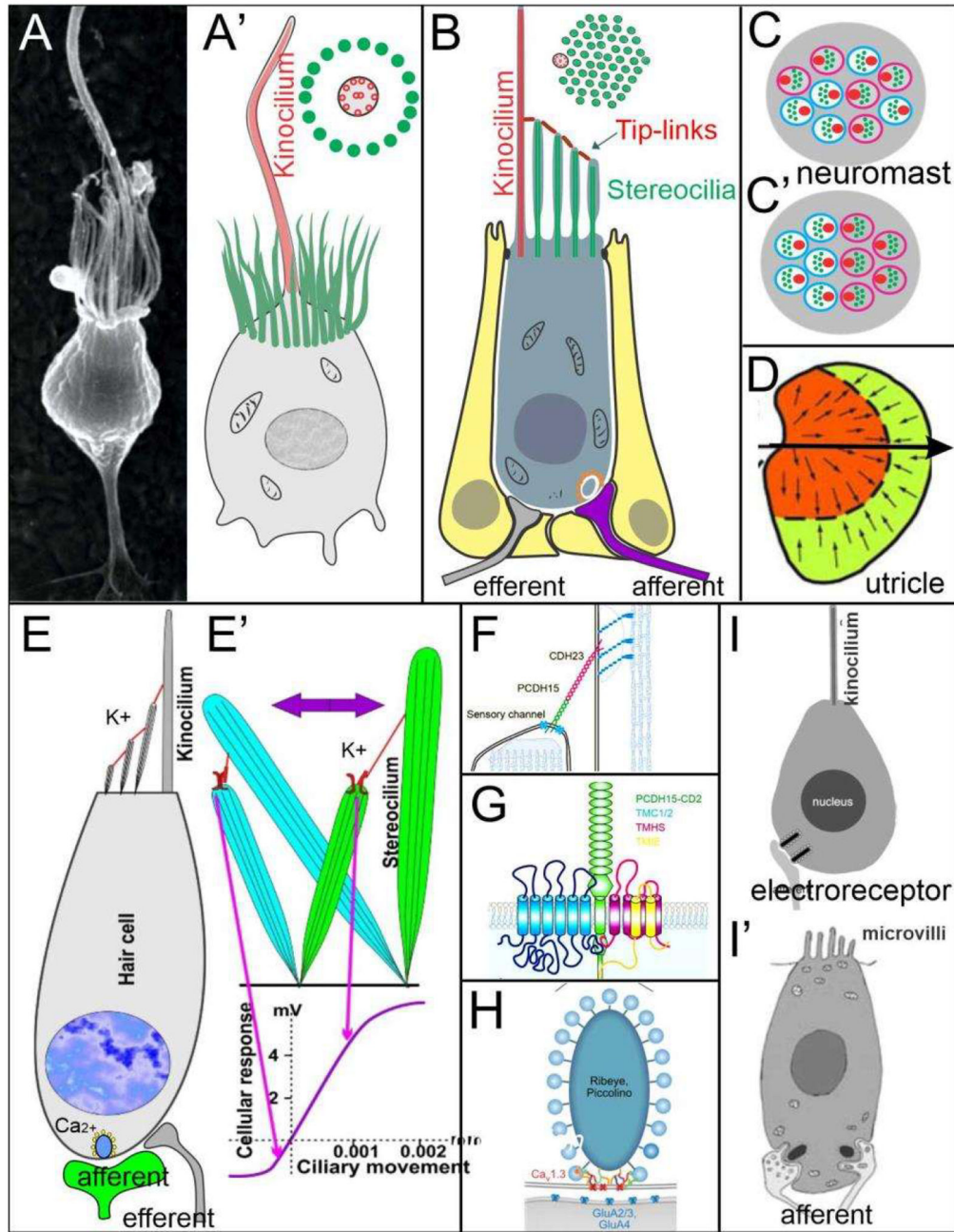
Figure 5. Mechanosensory hair cells evolve from single-cell organisms. Choanoflagellate ( A,A' ) are the basis of animals that evolved from a kinocilium surrounded by microvilli into an asymmetric staircase of mechanosensory hair cells ( B,C,E ) that forms the mechano-electrical transduction channels (MET) of the lateral line ( B,C,C' ) and vestibular hair cells ( E ). The lateral line ( C,C' ) and some vestibular hair cells ( D ) are bipolar, whereas canal cristae and most auditory organs are polarized in 1 direction. Tip links depend on CDH23 and PCDH15 ( F ) that interact with Tmc and others ( G ) to open up the channel ( E' ) to allow K + entrance. Ca 2+ interactions with t ribbons to allow the release of glutamate ( E,H ). Electroreceptors
