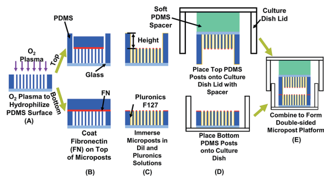
Fig. 1 Schematic of fabrication technology for double-sided micropost platform to measure cell traction force in confined space. Effects of confinement and contact area were studied by modifying separation height and density of micropost arrays on top and bottom. (A) Using O 2 plasma to hydrophilize polydimethylsiloxane (PDMS) microposts for coating fibronectin (FN). (B) Coating FN on top of microposts. (C) Blocking cell adhesion on sidewalls of microposts by covering sidewalls with Pluronic F-127 and labeling microposts with red stain Dil to enhance imaging contrast. (D) Placing top micropost platform on soft PDMS spacer and bonding to lid of 35 mm diameter (dia.) cell culture dish. Bottom micropost platform was placed on cell culture dish. (E) After seeding MC3T-E1 cells on bottom micropost platform, two parts were sealed to form double-sided micropost platform.
