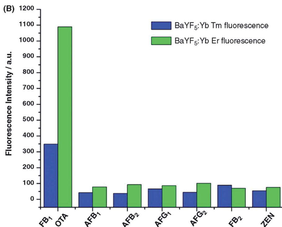
Fig. 35 (A) Schematic representation of the immobilization of ochratoxin A (OTA) aptamers and fumonisin B1 (FB1) aptamers and their multiplex upconversion FRET between aptamer-UCNPs and GO for detecting OTA and FB1. (B) Fluorescence signal change for different mycotoxins at a concentration of 10 \text{ ng mL}^{-1} . FB1 and OTA show a significant increase in fluorescence intensity compared with other mycotoxin homologs, including AFB1, AFB2, AFG1, AFG2, fumonisin B2 (FB2) and zearalenone (ZEN), which are commonly found in foods. [Reprinted with permission from ref. 682, S. Wu, N. Duan, X. Ma, Y. Xia, H. Wang, Z. Wang and Q. Zhang, Multiplexed Fluorescence Resonance Energy Transfer Aptasensor between Upconversion Nanoparticles and Graphene Oxide for the Simultaneous Determination of Mycotoxins, Anal. Chem. , 2012, 84 , 6263–6270. Copyright© American Chemical Society.]
