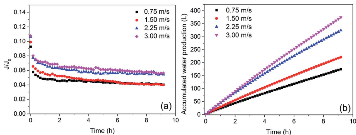
Fig. 5 Effect of CFV on permeate flux (a) and water production (b) (CF = 1, temperature = 18 \pm 2 °C, TMP = 2.20 bar).
