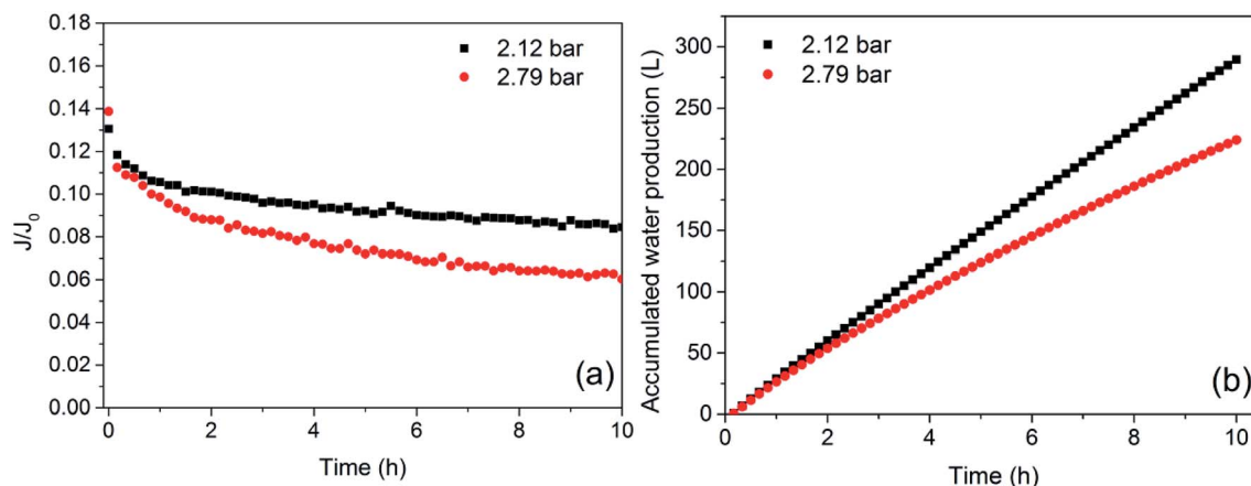
Fig. 4 Effect of TMP on permeate flux (a) and water production (b) (CF = 1, temperature = 18 \pm 2 °C, CFV = 2.50 \text{ m s}^{-1} ).
