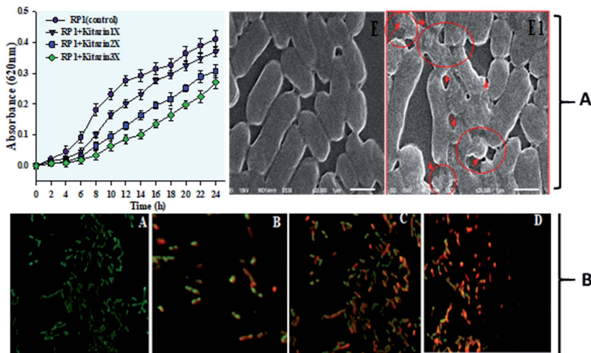
Fig. 3 Depicts the growth pattern of R. leguminosarum strain RP1 grown in minimal medium supplemented with increasing concentrations of kitazin as a function of time of incubation at 28 \pm 2 °C. Data represent the mean \pm S. D of three independent experiments done in triplicate (A). Control and kitazin treated SEM micrograph of strain RP1 (red coloured arrows indicate the damage/rupture in cells after exposure to kitazin (A)). CLSM images of live/dead cells of R. leguminosarum strain RP1 stained with AO/PI indicating the cell viability (A) control (B–D) treated with 600, 1200 and 1800 \mu\text{g mL}^{-1} kitazin (B).
