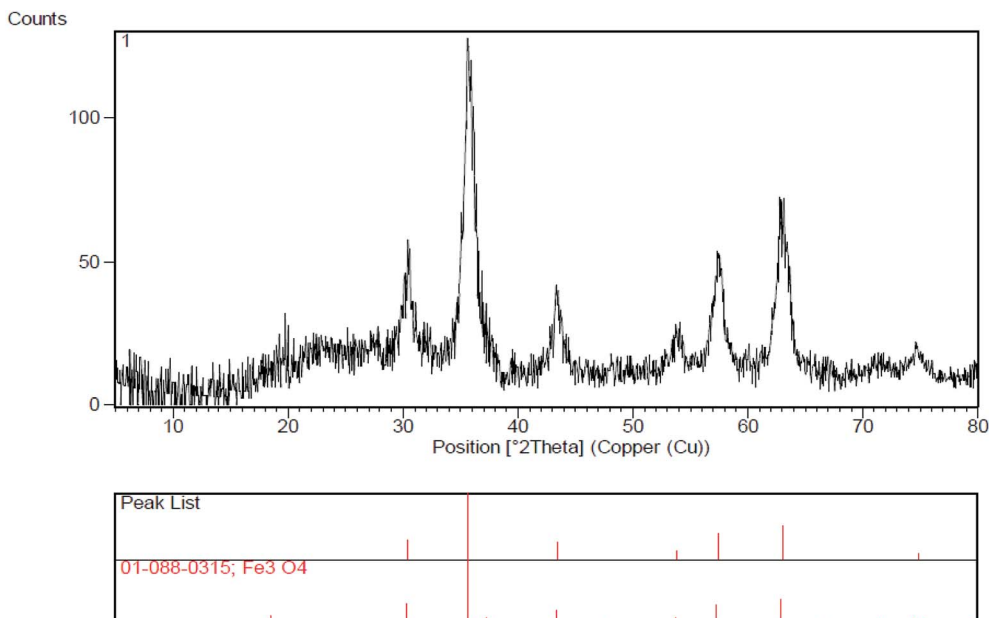
Fig. 10 XRD pattern of recovered Fe 3 O 4 /SO 3 H@zeolite-Y.
