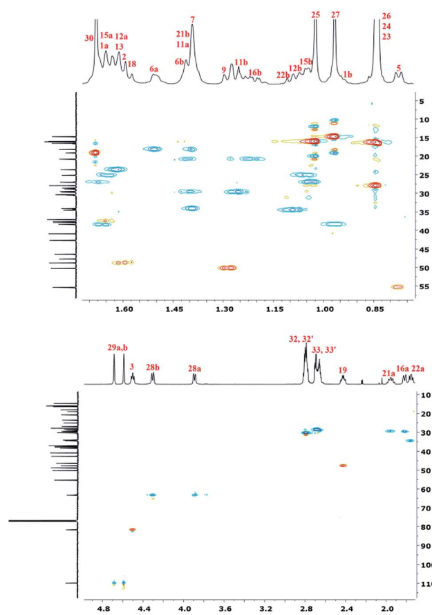
Fig. 7 HSQC NMR spectrum of polyDBB.
