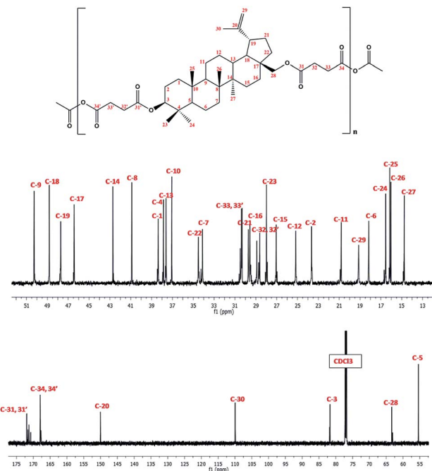
Fig. 6 13 C NMR spectrum of polyDBB.
