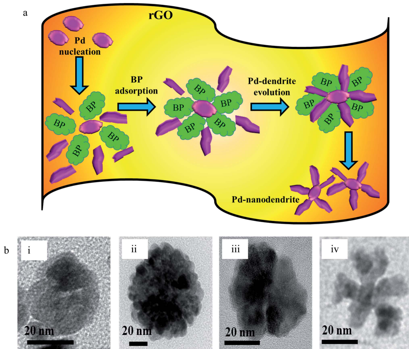
Scheme 2 (a) Representative diagram of the mechanism of synthesis of PRGO-nd in the presence of BP. (b) TEM images of Pd NPs deposited on rGO using (i) acetone, (ii) hydroquinone, (iii) acetophenone, and (iv) BP.
