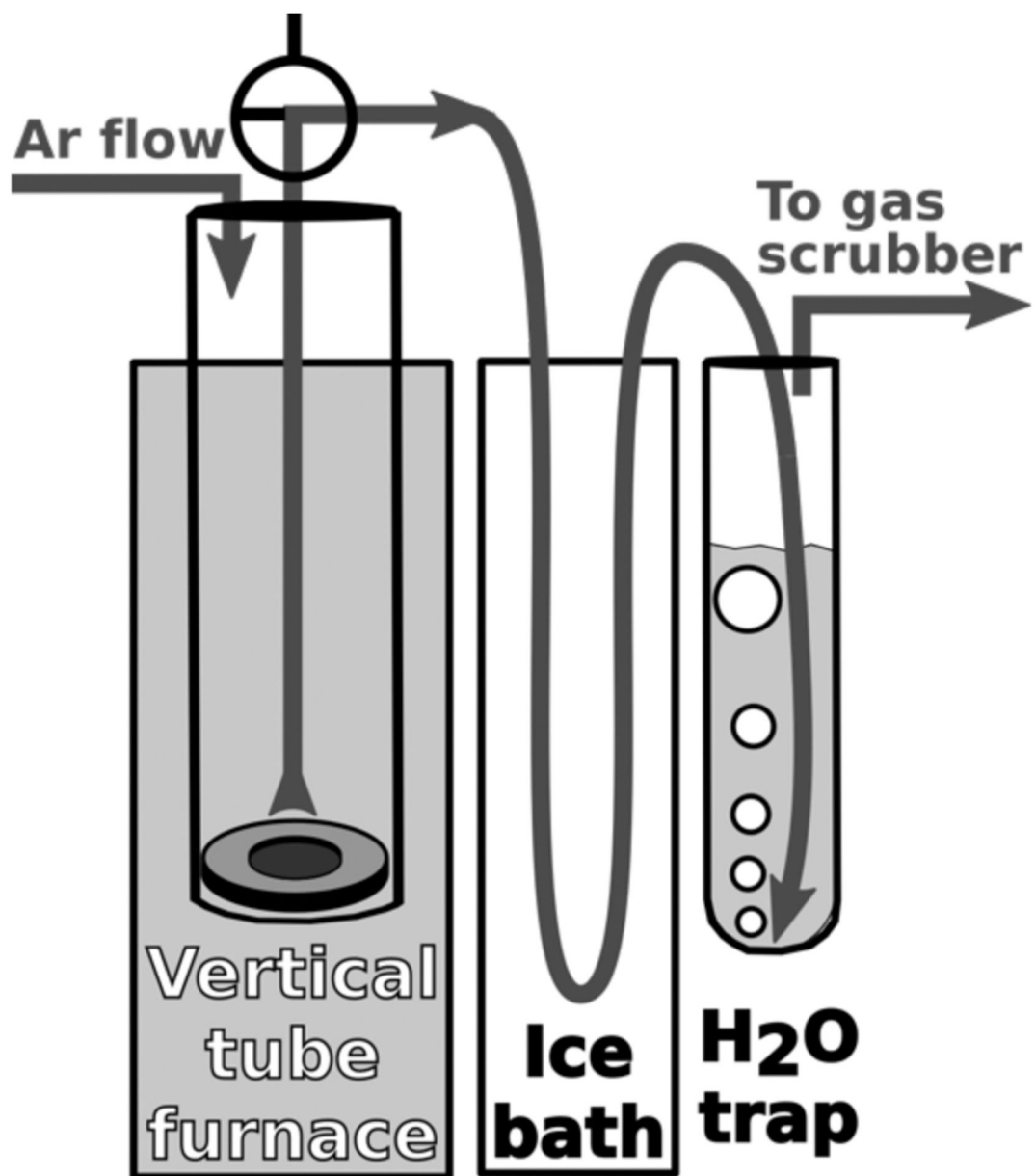
Figure 1. Radiobromine furnace assembly with CoSe heated inside quartz tube (left).
