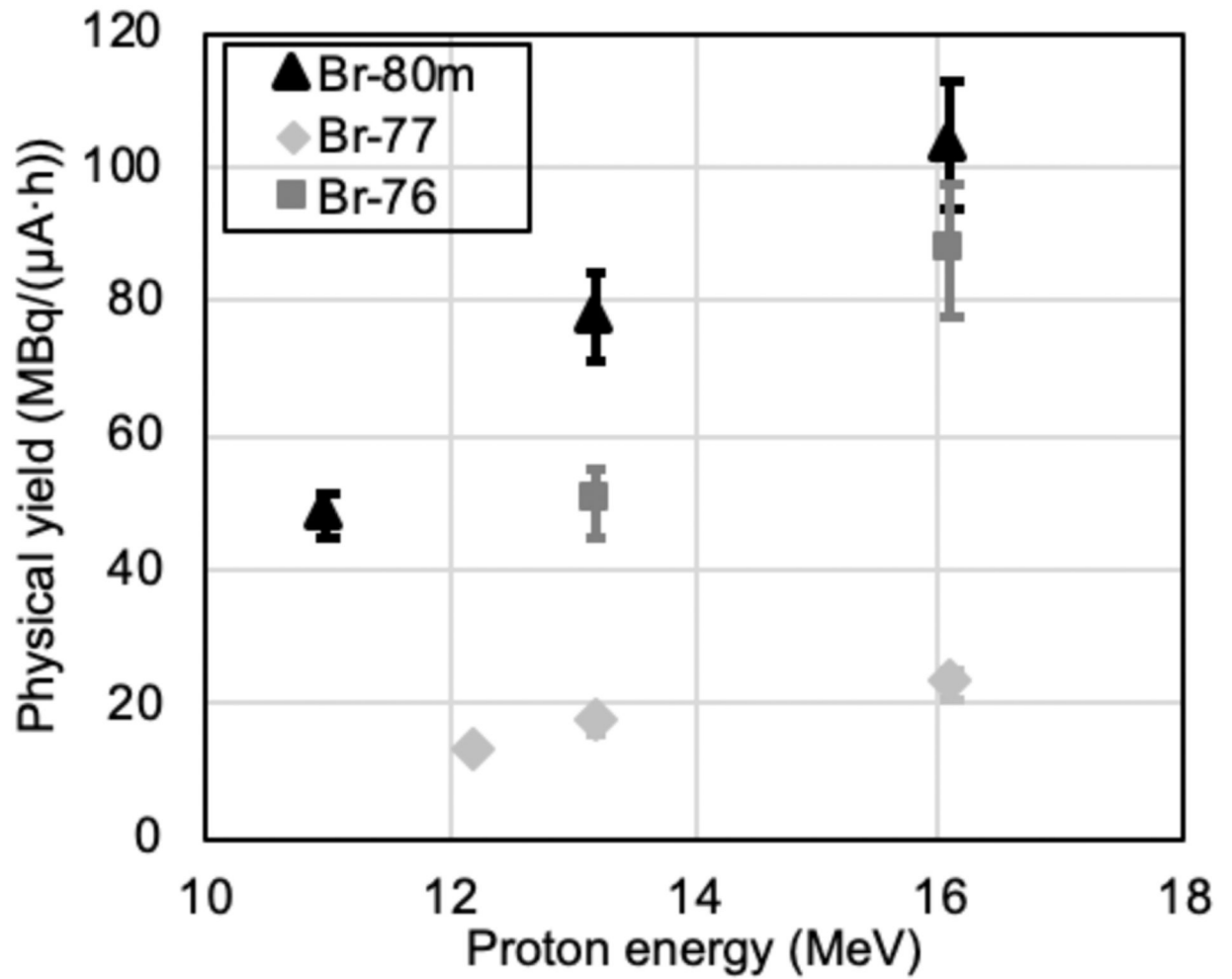
Figure 3. Production yield of ^{80\text{m}}\text{Br} , ^{77}\text{Br} , and ^{76}\text{Br} from irradiation of \text{Co}^{80}\text{Se} , \text{Co}^{77}\text{Se} , and \text{Co}^{76}\text{Se} , respectively. Error bars represent standard deviations of measurements from multiple irradiations (see Table 1 for details).
