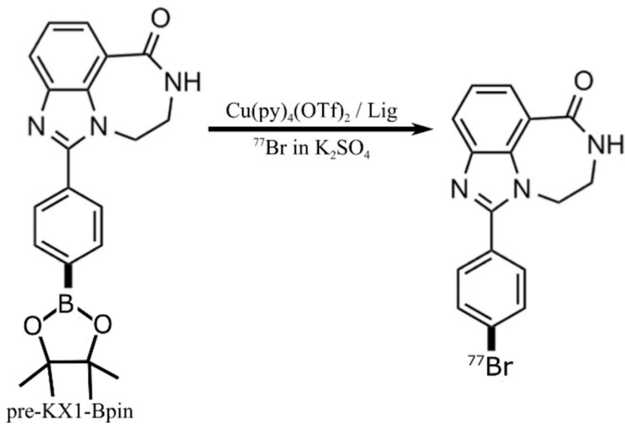
Figure 2. Radiosynthesis of ^{77}\text{Br} -labeled PARP-1 inhibitor.
