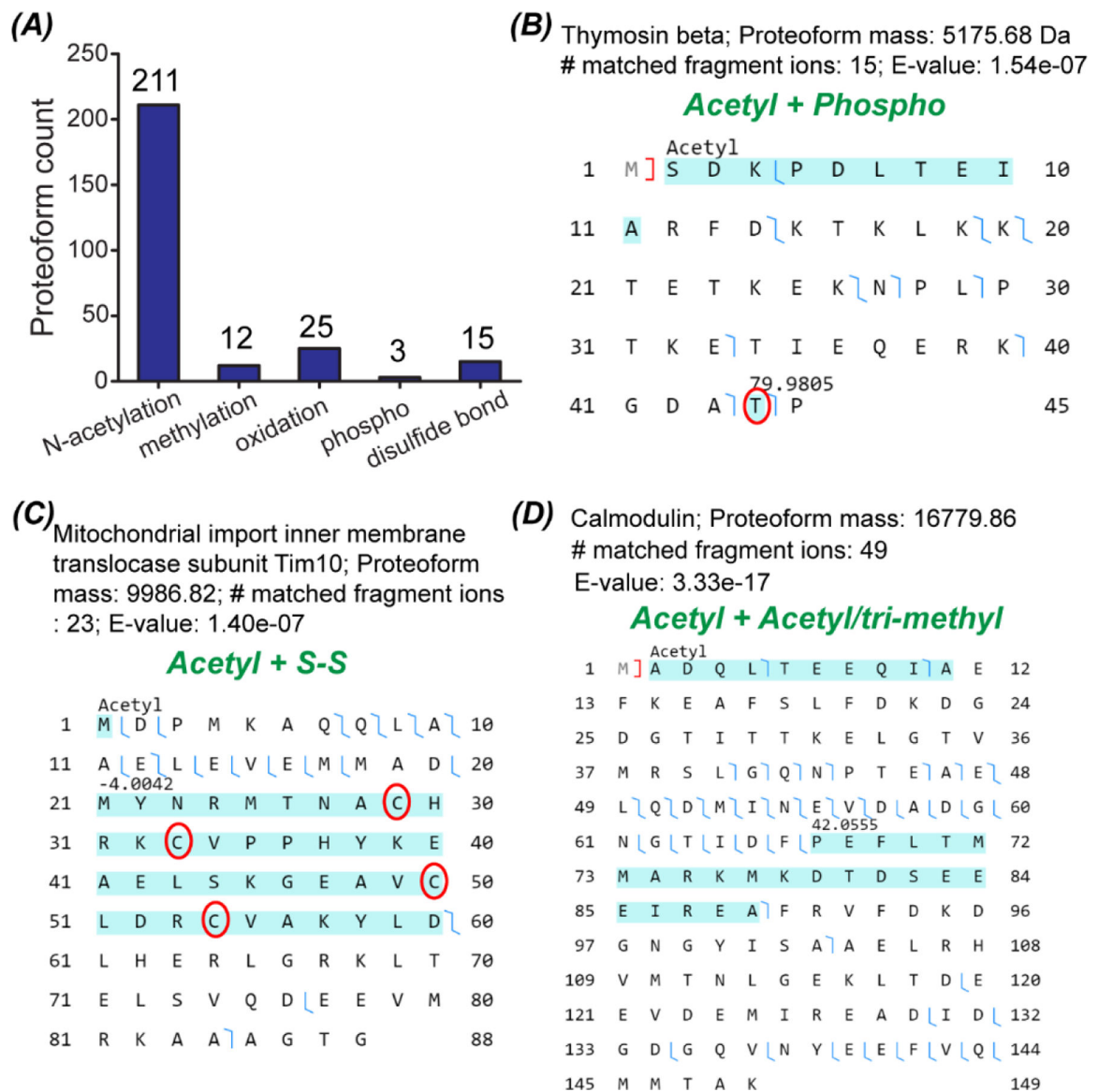
Fig. 5. Data about proteoforms with PTMs. (A) The number of proteoforms with various PTMs identified from the Tel2 and Teo2 samples. (B–D) Sequences and fragmentation patterns of three proteoforms with combinations of various PTMs.
