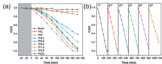
Fig. 7 (a) Photocatalytic performances of TiO 2 , TF0, TF0.1, TF0.2, TF0.5, TF1.0, TF2.0 and Fe 2 O 3 for reduction of Cr(vi) under visible light irradiation. (b) Cyclic photoreduction Cr(vi) experiments of TF0.5.
