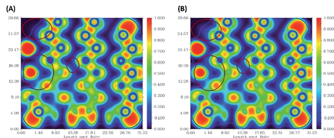
Fig. 6 Electron-density images of some phosphorus atoms present in phosphorene: (A) ELF for phosphorene, (B) ELF for phosphorene present in phosphorene-chlorambucil.
