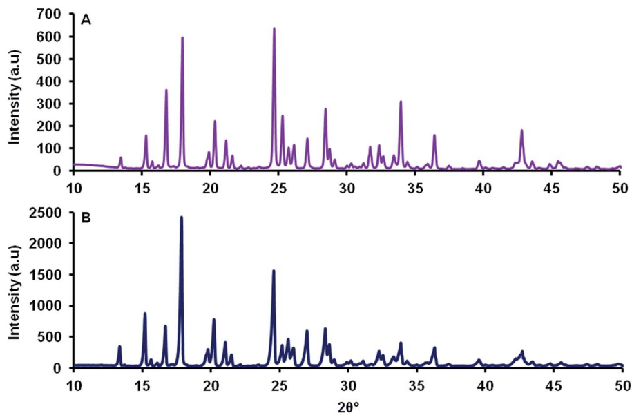
Fig. 2 Unrefined powder diffraction patterns of MCT® (A) and L-tyr (B) determined over the range 10–50 2\theta^\circ .
