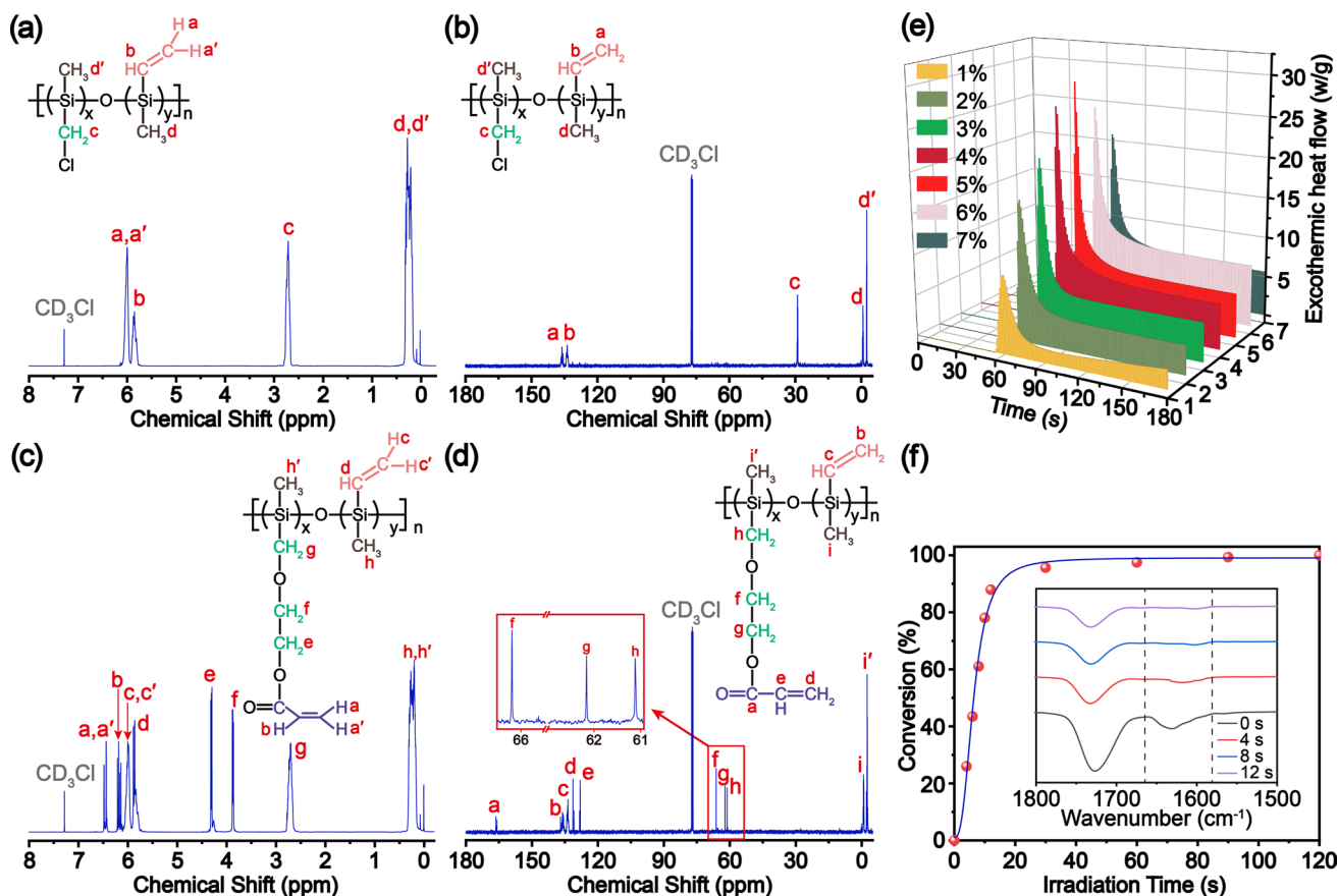
Fig. 2 Structural characterization of the PSO and UV-PSO precursors: a, c ^1\text{H} NMR spectra; b, d ^{13}\text{C} NMR spectra; e DPC thermograms of UV-PSO with different photoinitiator concentrations; and f conversion percentage of acrylic group at different curing times (inset with FT-IR spectra)
