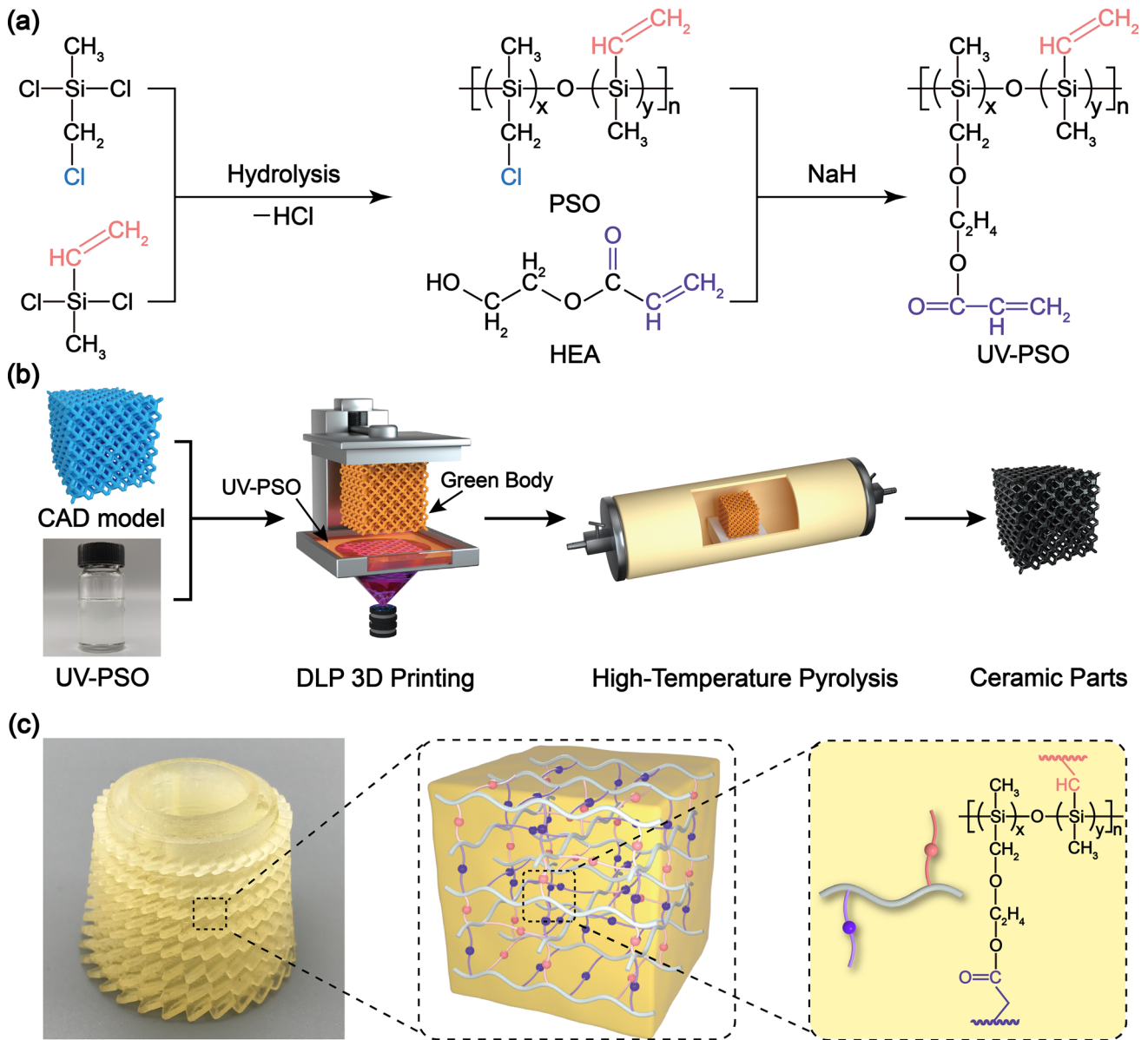
Fig. 1 Synthesis route of the UV-curable polysiloxane and schematic DLP printing process and preparation of the designed Si–O–C ceramic metamaterial: a synthesis route of UV–PSO; b 3D printing of UV–PSO and pyrolysis process of Si–O–C ceramic metamaterial; and c photograph of a representative booster blade DLP-printed green body and two kinds cross-linked molecular structure of the UV–PSO
