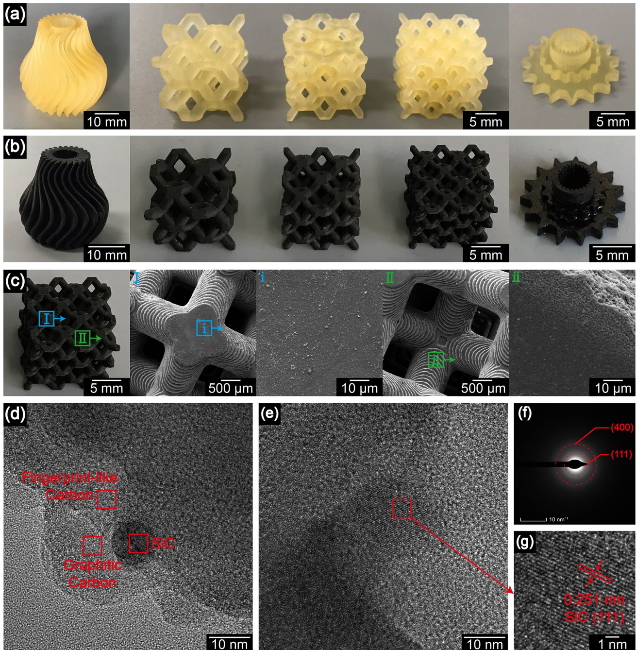
Fig. 3 Morphology and structures of 3D-printed green bodies and the corresponding pyrolytic ceramics: a typical structure of green bodies prepared by the DLP 3D printing; b corresponding structure of Si–O–C ceramic parts; c surface morphology SEM images of the ceramic cell structure; d , e TEM images; f selected area electron diffraction (SAED) image; and g lattice fringe of SiC
