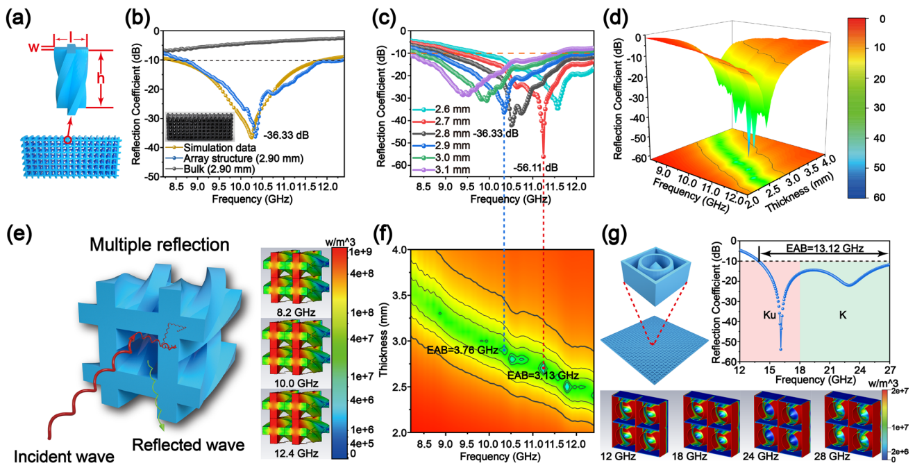
Fig. 4 Design and fabrication of Si–O–C ceramic metamaterial structure in X-band: a unit and array structure models; b calculated RC values of the bulk sample, array structure sample, and the simulated data of the array structure; c RC versus frequency and thickness corresponding to d 3D graph and f 2D projection diagram; e multiple reflection mechanism; and g metamaterials structure design suitable for Ku and K bands
