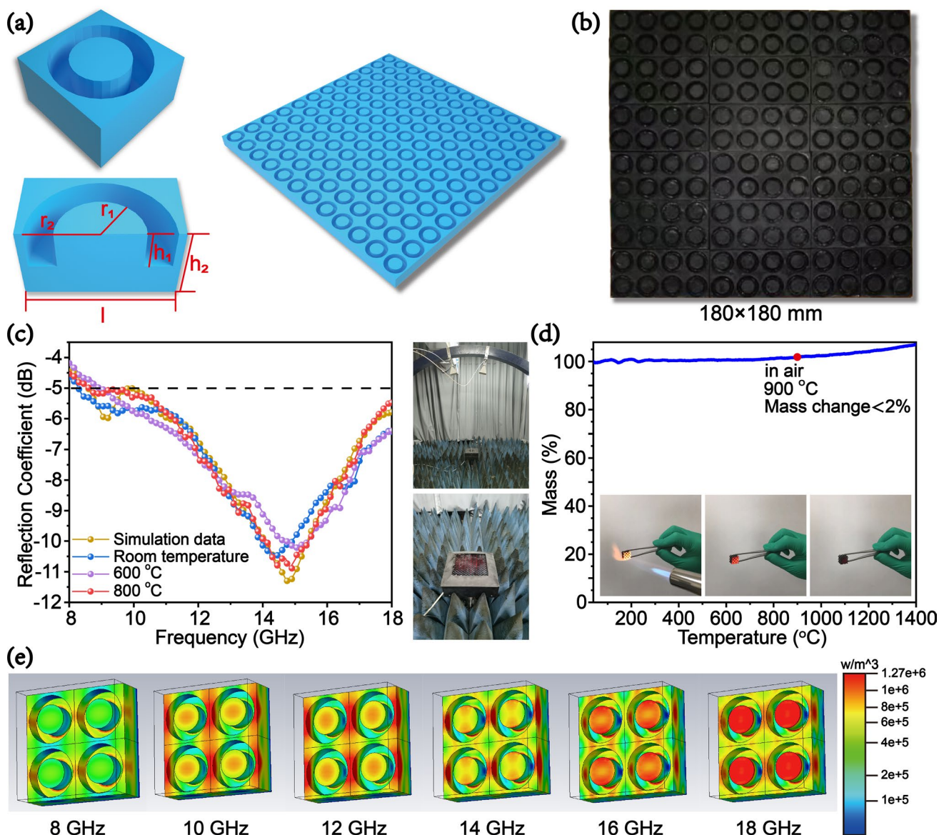
Fig. 5 Design and fabrication of Si–O–C ceramic metamaterial structure for practical application in X–Ku band: a unit and array structure models; b actual photograph of the sample; c comparison of the measured RC data at different temperatures and simulation data; d high-temperature oxidation resistance of Si–O–C ceramic parts; and e energy flow density of the simulated array structure at different frequencies
