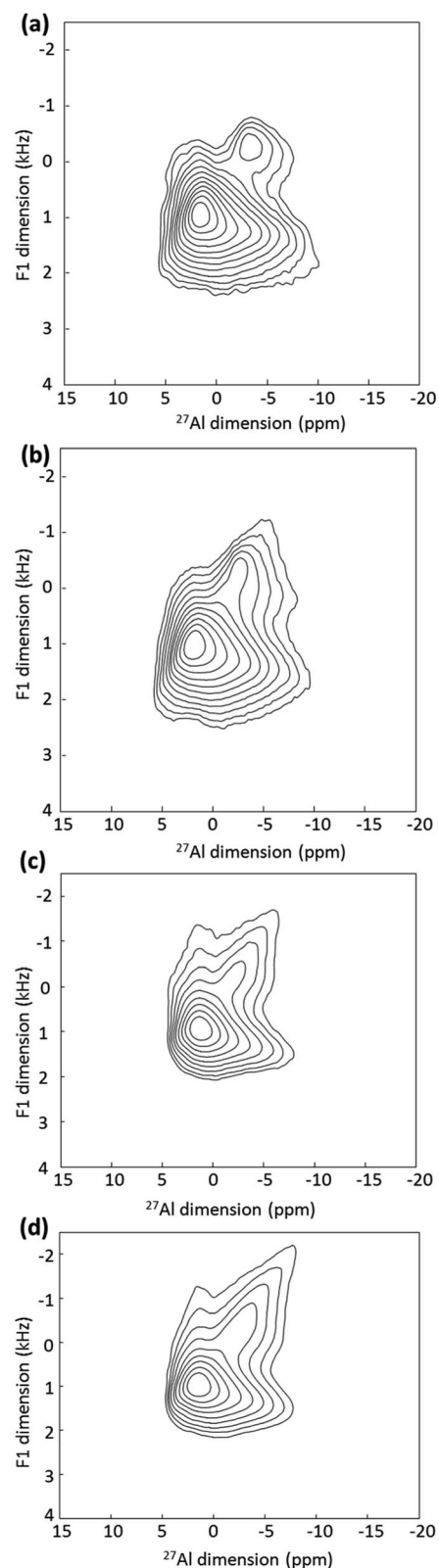
Fig. 2 27 Al MQMAS NMR spectra of (a) pristine nanoMIL-100(Al) and nanoMIL-100(Al) (b) coated with CD-P, (c) loaded with ATP and (d) loaded with ATP and coated with CD-P.
