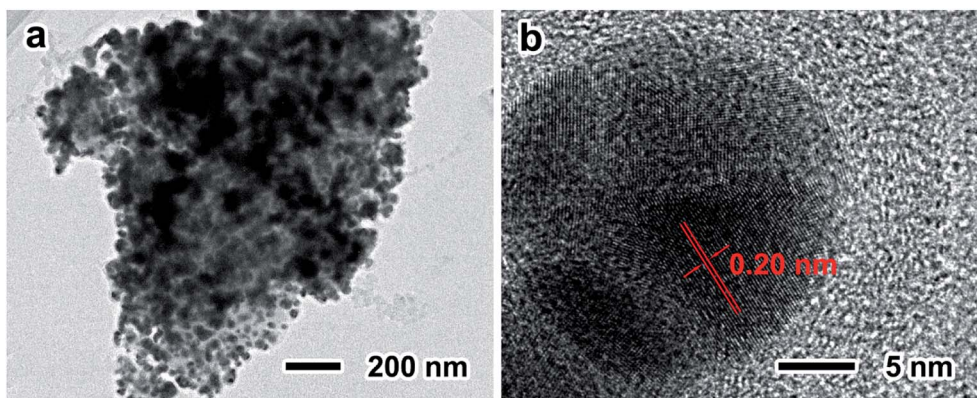
Fig. 6 Low- (a) and high-magnification TEM (b) images of TS-P-Si after 50 cycle times at a current density of 400 \text{ mA h g}^{-1} .
