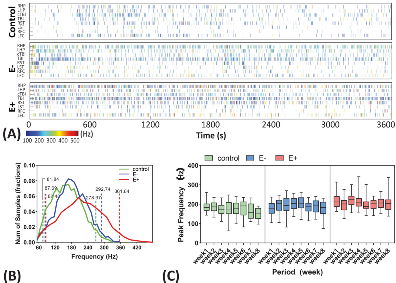
Fig. 2. Peak frequency distributions and consistency. (A) HFO events presented in a selected 1-hour file from control, E- and E+ group in the 8 brain recording sites. Each bin represents a HFO events with the color indicates the peak frequency (blue- low, red- high). Abbreviations are similar to those in the Fig. 1). (B) HFO peak frequency distribution in control, E- and E+ group. The range of HFO was plotted between 60 and 480 Hz. Control, E- and E+ group showed a mean peak frequency of 170.9, 190.2 and 219.1 Hz. Dashed lines represent the 95% confidence of interval of the mean. E+ group were found significantly larger than E- and control group at the alpha = 0.05. No differences were found between control and E- group. (C) Consistency of the HFO peak frequency presented as group × weeks. No within-group differences were found for all three group in the 8-week test period. (For interpretation of the references to color in this figure legend, the reader is referred to the web version of this article.)
