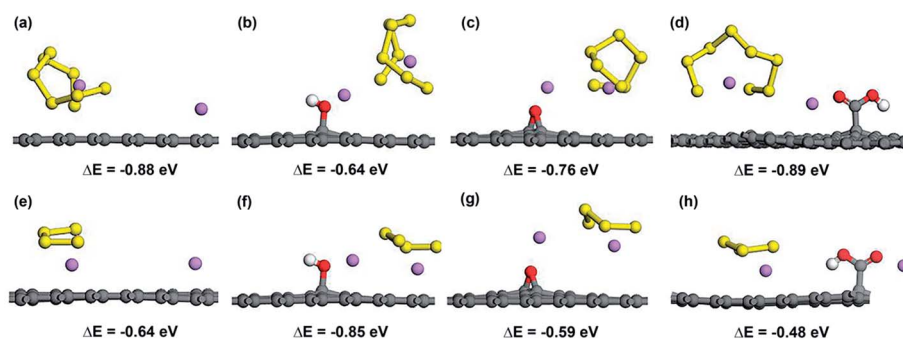
Fig. 7 Atomic configurations and \Delta E values of Li + \text{LiS}_8 and Li + \text{LiS}_4 clusters adsorbed on graphene (a and e), hG (b and f), eG (c and g) and cG (d and h) respectively.
