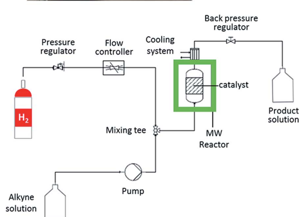
Fig. 2 (a) MW flow reactor for alkyne semi-hydrogenation. (b) Scheme of MW continuous flow reactor setup for liquid-phase catalytic alkyne hydrogenation reaction.
