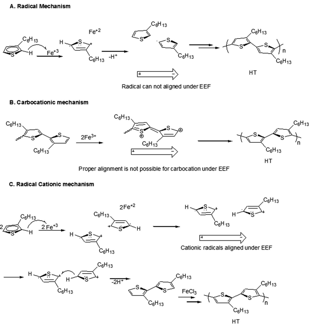
Scheme 2 Possible mechanisms of polymerization reaction.
