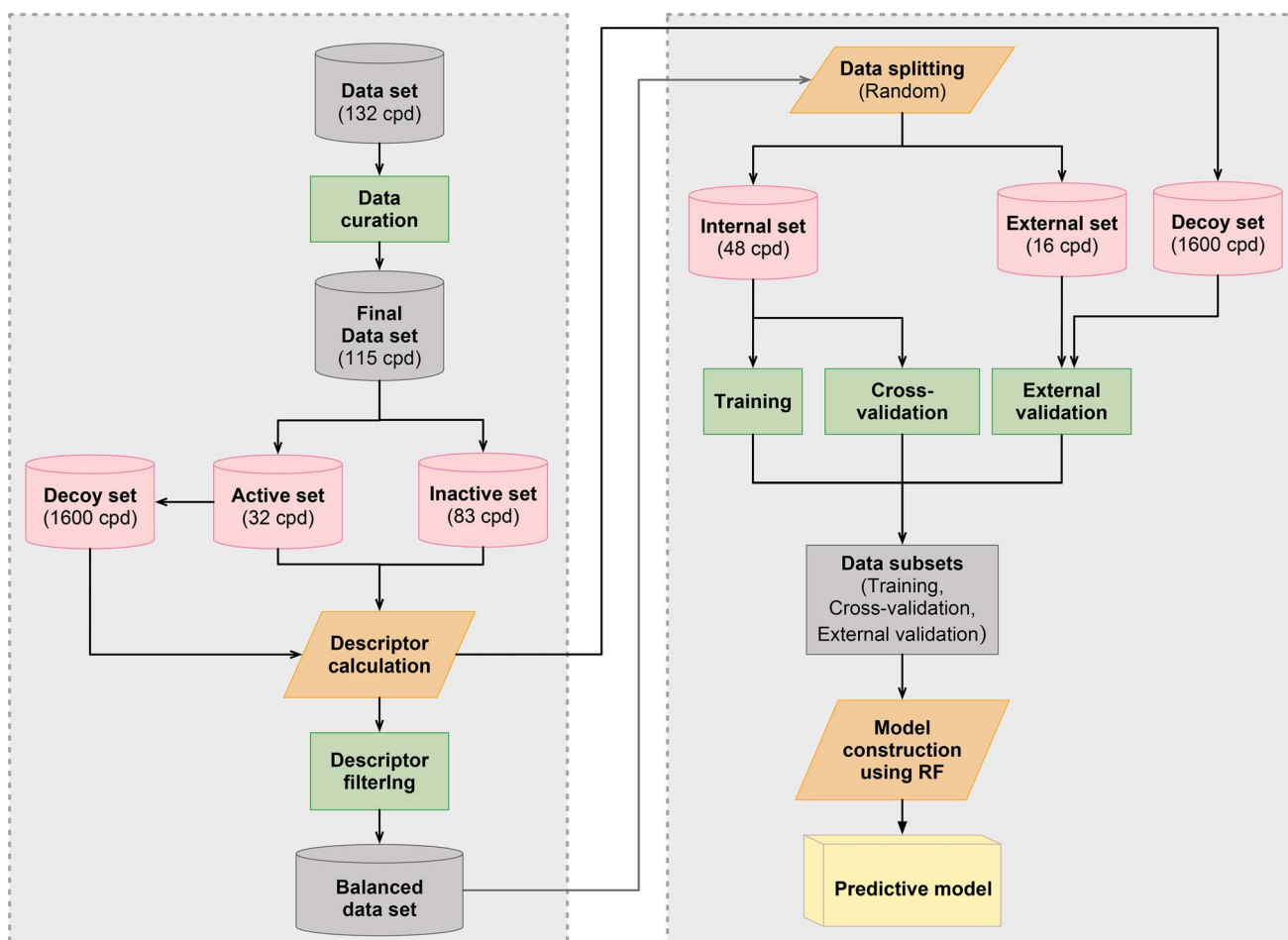
Fig. 2 Workflow of CSAR modeling for investigating anti-sickling activity.
