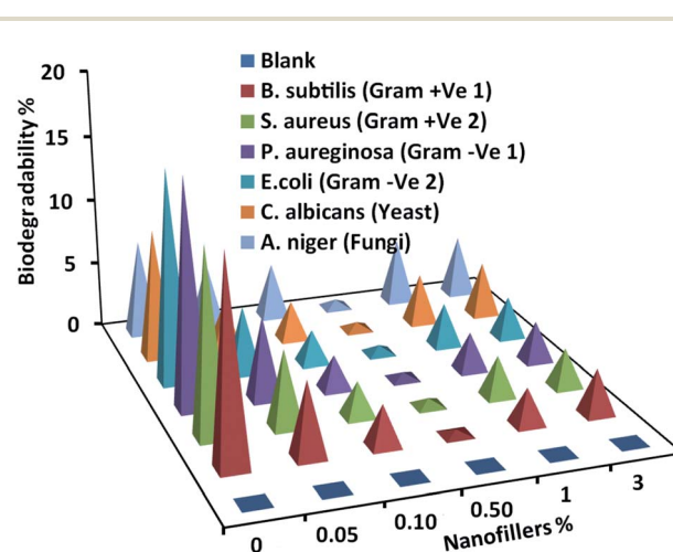
Fig. 7 Biodegradability determinations of the virgin silicone and PDMS/spherical Ag@SiO 2 core-shell nanocomposites against different micro-foulants.
